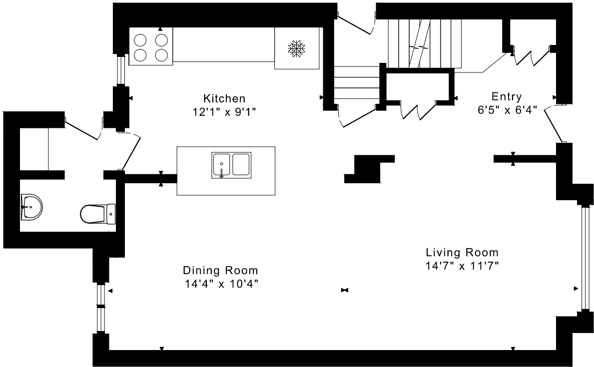
MAIN FLOOR 715 SQUARE FEET
