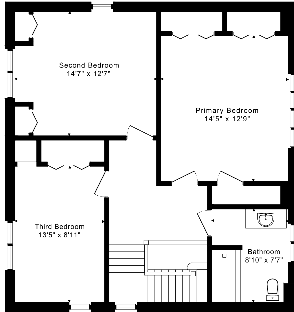
SECOND FLOOR 905 SQUARE FEET
