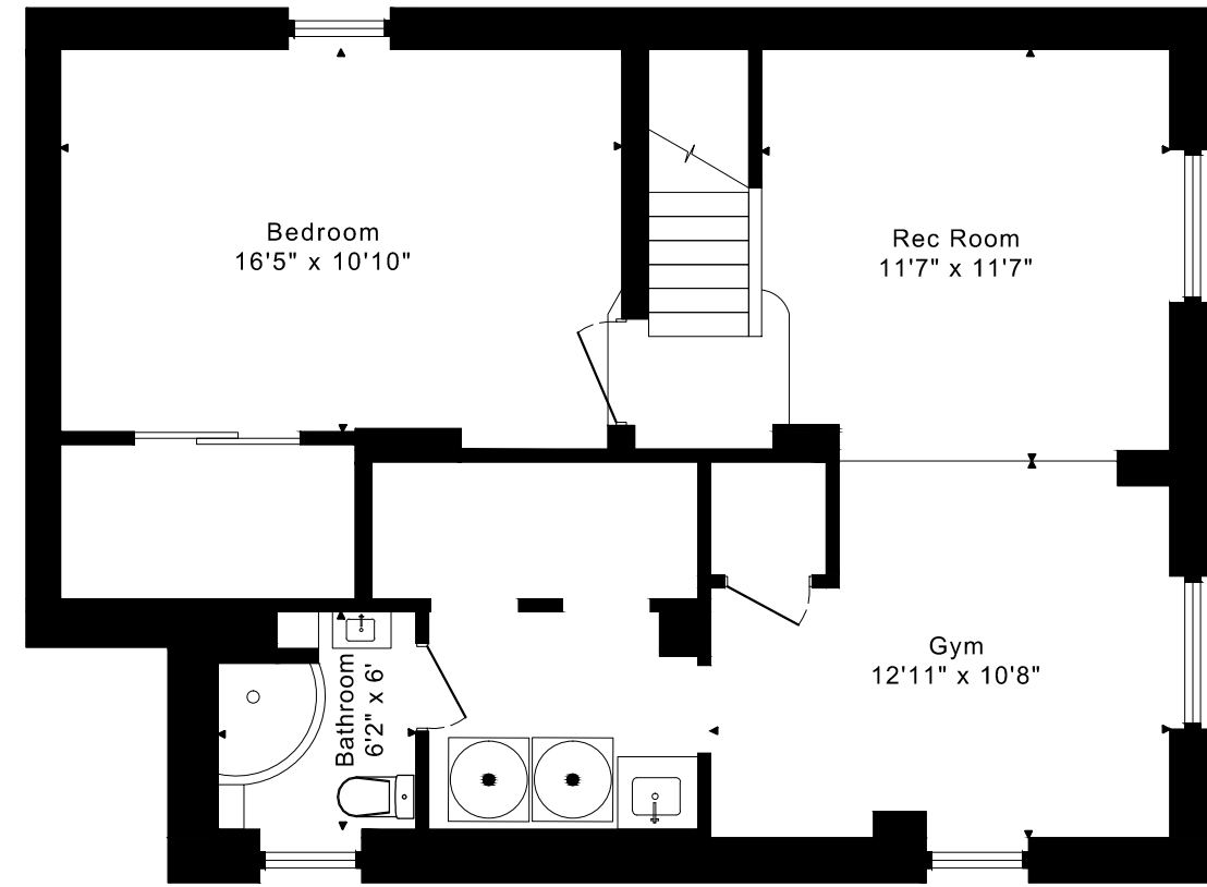
LOWER FLOOR 805 SQUARE FEET
