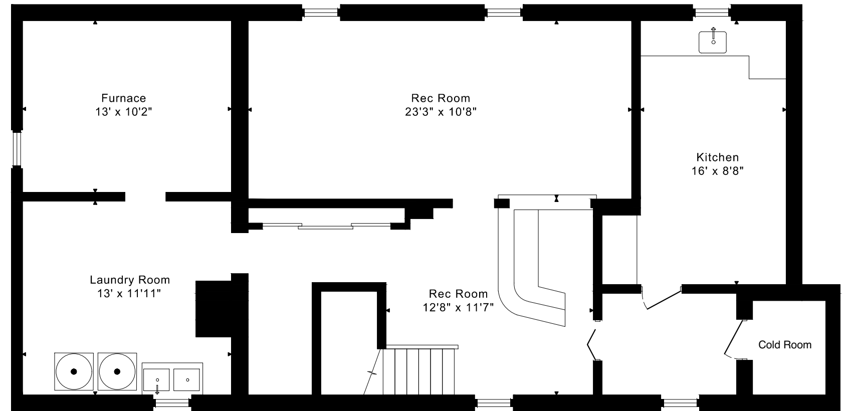
LOWER FLOOR 1225 SQUARE FEET
