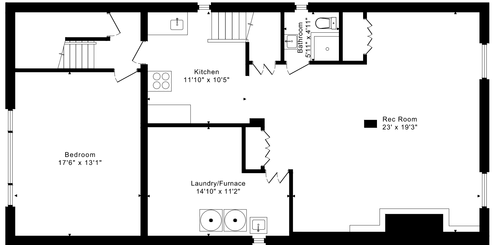
LOWER FLOOR 1285 SQUARE FEET
