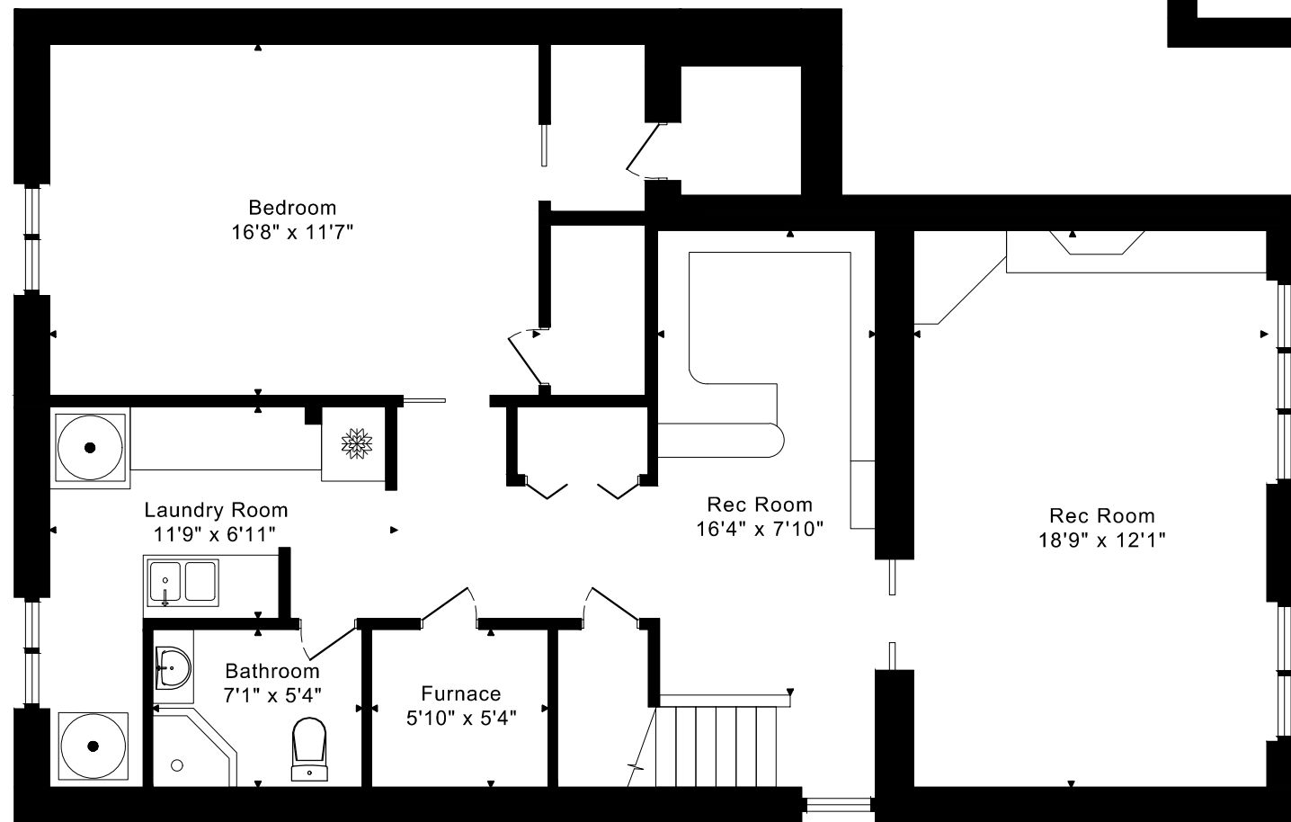
LOWER FLOOR 1120 SQUARE FEET
