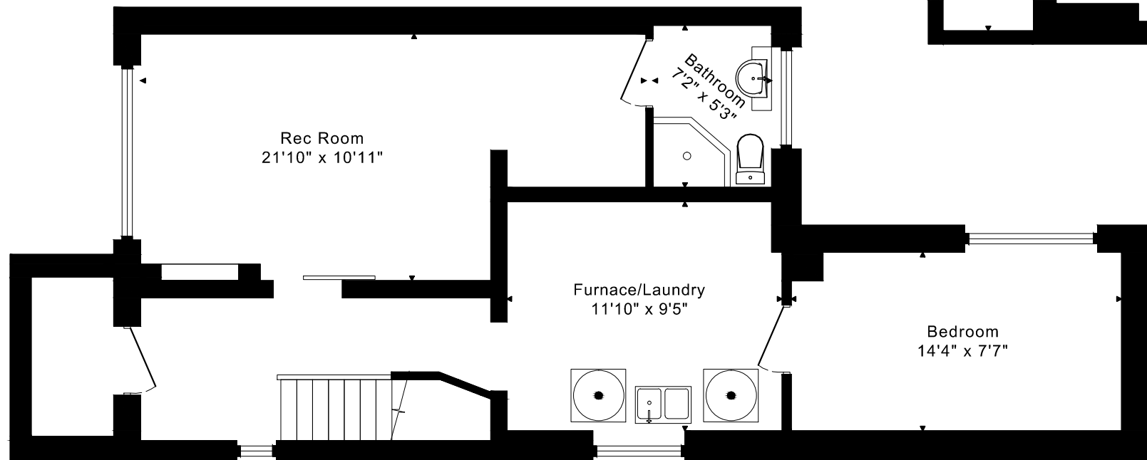
LOWER FLOOR 780 SQUARE FEET
