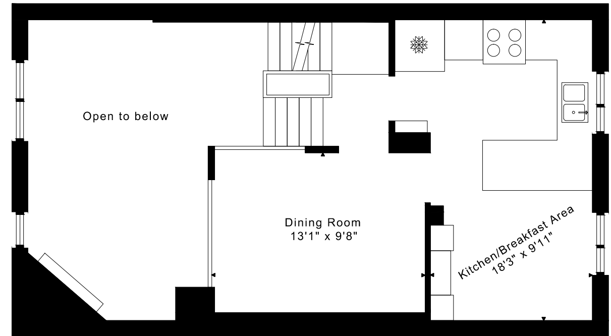
SECOND FLOOR 470 SQUARE FEET
