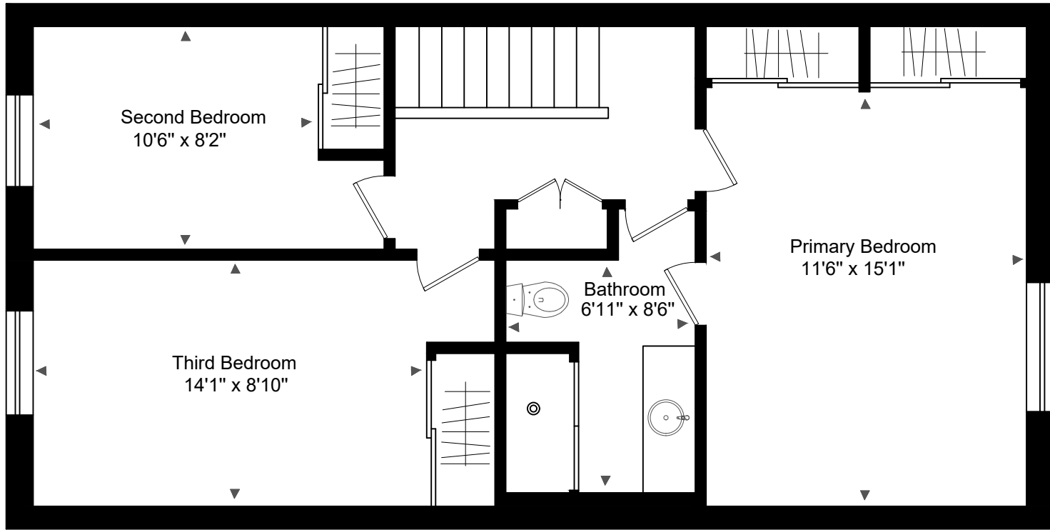
SECOND FLOOR 680 SQUARE FEET
