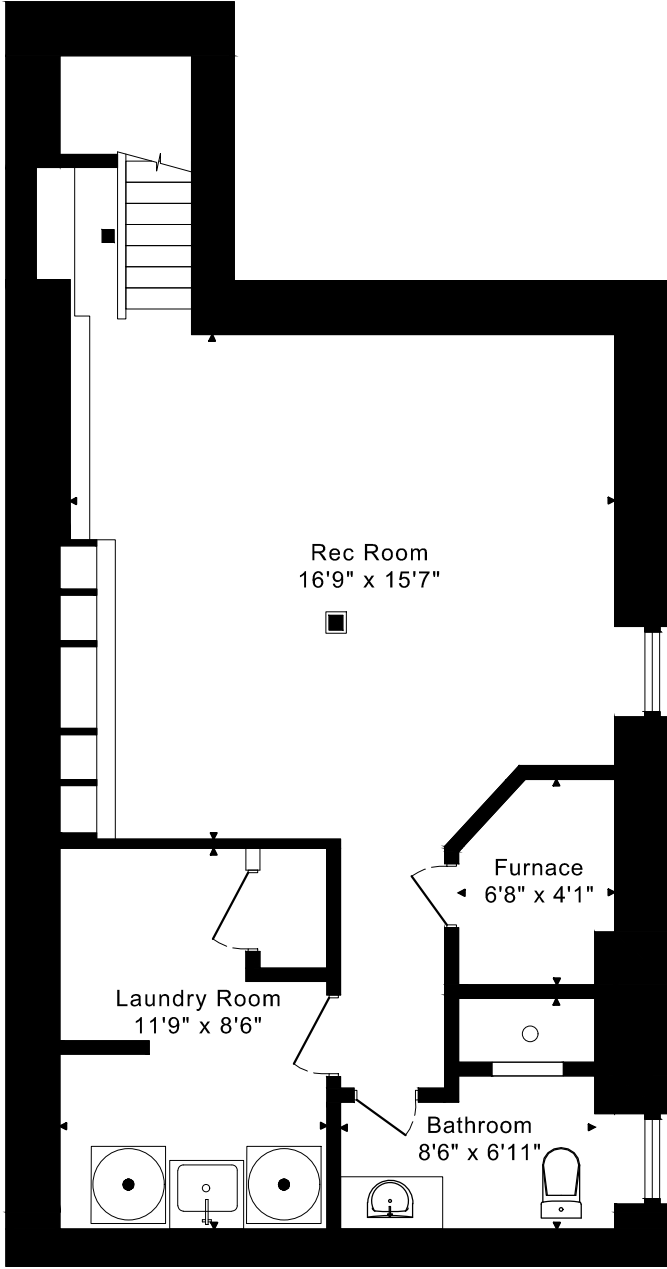
LOWER FLOOR 675 SQUARE FEET
